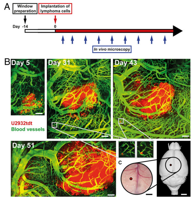
Fig. 1. Characteristic pattern of PCNSL growth repeatedly visualized with in vivo TPLSM. (A) Schematic representation illustrating experimental design. (B) Intracerebral tumor growth after stereotactic implantation of U2932tdt cells (red). Blood vessels are highlighted after i.v. injection of FITC-dextran (green). Images represent mosaics of multiple maximum intensity projections. Insets show perivascular, dormant tumor cells. Representative mosaics of 15 mice from 8 independent experiments. (Scale bars: 100 μm.) (C) Position of tumor implantation (red) and position and dimensions of the chronic cranial window (circle; 6 × 6 mm). (Scale bars: Left, 1 mm; Right, 2 mm.) Right panel created with 3dBAR plugin of the Scalable Brain Atlas (SBA) (53–55).
